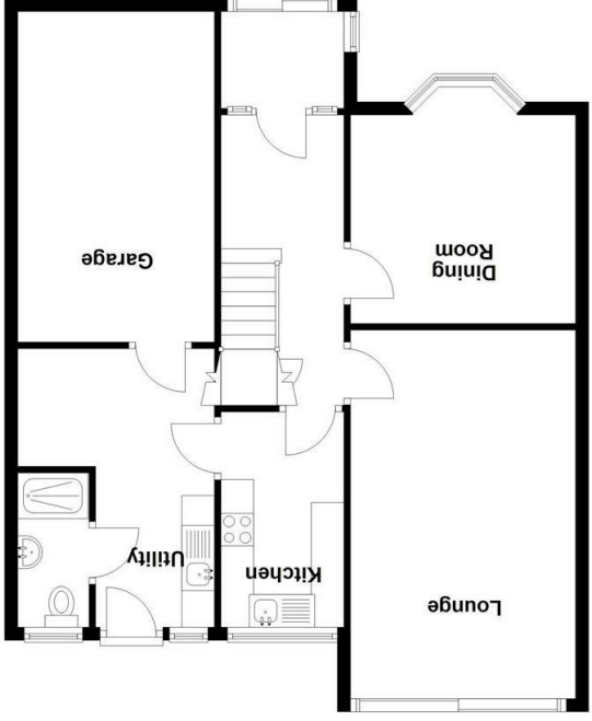
Ground Floor Approx. 78.9 sq. metres (849.6 sq. feet)
